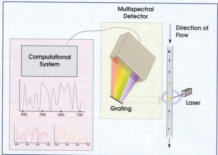
Figure 3. In a multispectral flow cytometer, a grating disperses signals from the fluorescence collector lens to a 32-channel Hamamatsu PMT. Detectors submit the data to the computational system, which determines hyperspectral curves for every particle and performs spectral unmixing.
